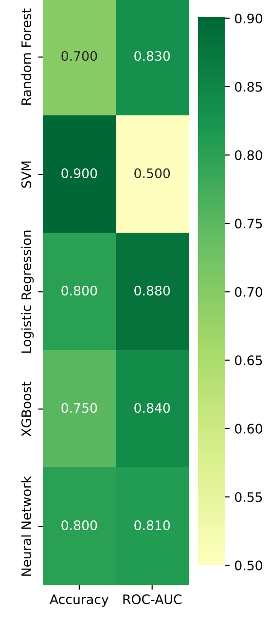
Model Performance Heatmap
