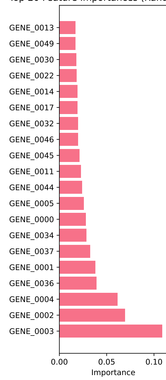
Top 20 Feature Importances (Random Forest)
